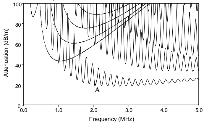
FIGURE 11. Attenuation dispersion curves for axially symmetric modes in 22mm diameter steel bar in limestone.
